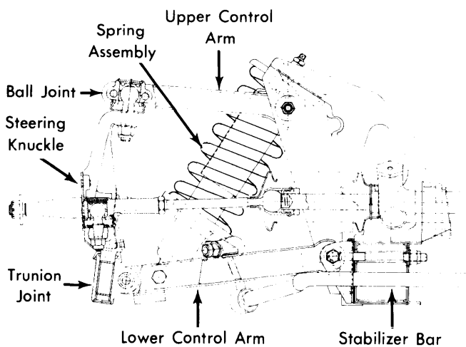
Fig. 1 Assembled View of Triumph Front Suspension
