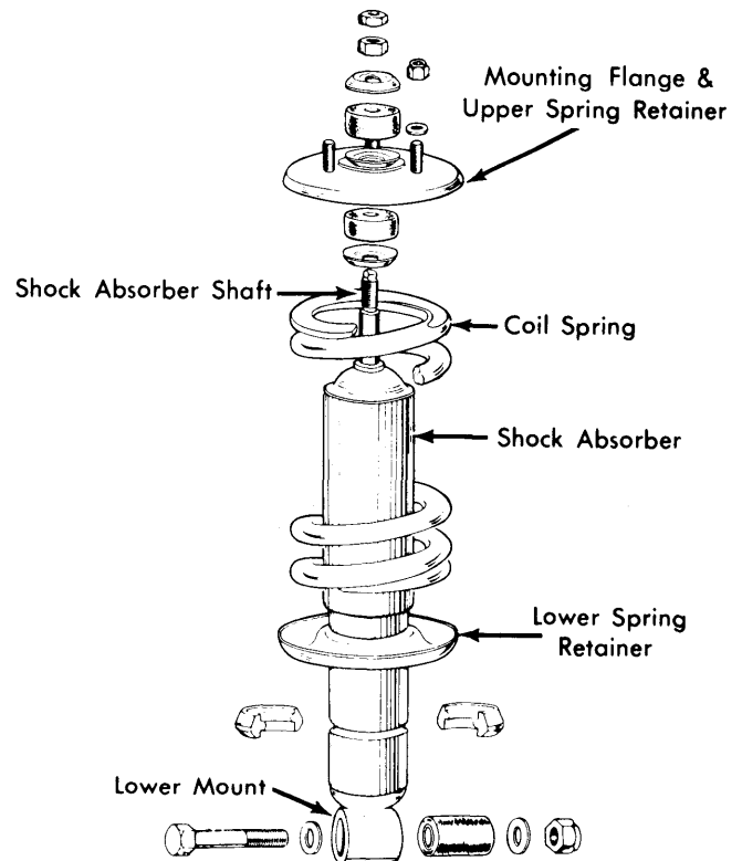
Fig. 2 Coil Spring and Shock Absorber Assembly
