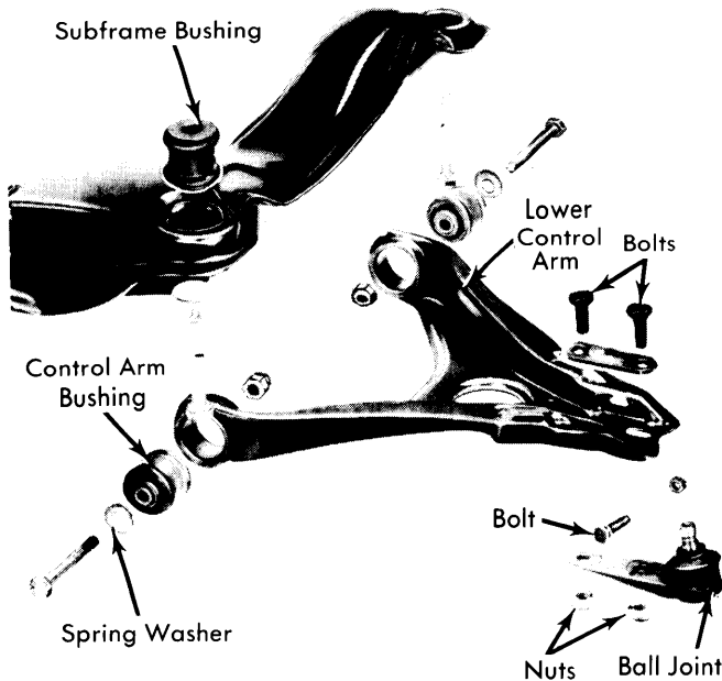
Fig. 2 Exploded View of Lower Control Arm Assembly
