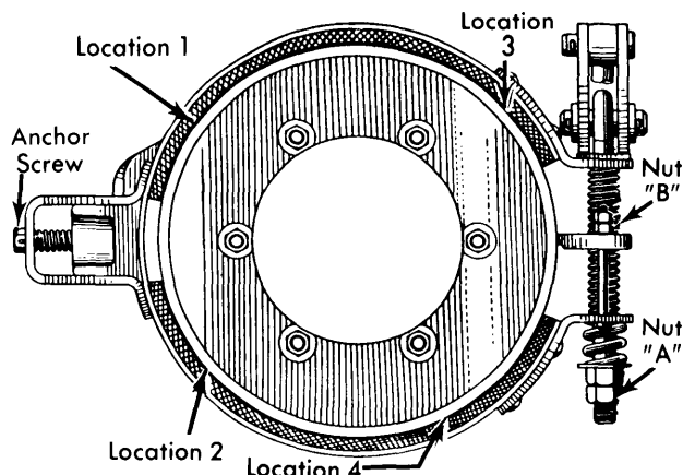
Fig. 2 Transmission Mounted External Contracting Anchor Pin Adjustment
