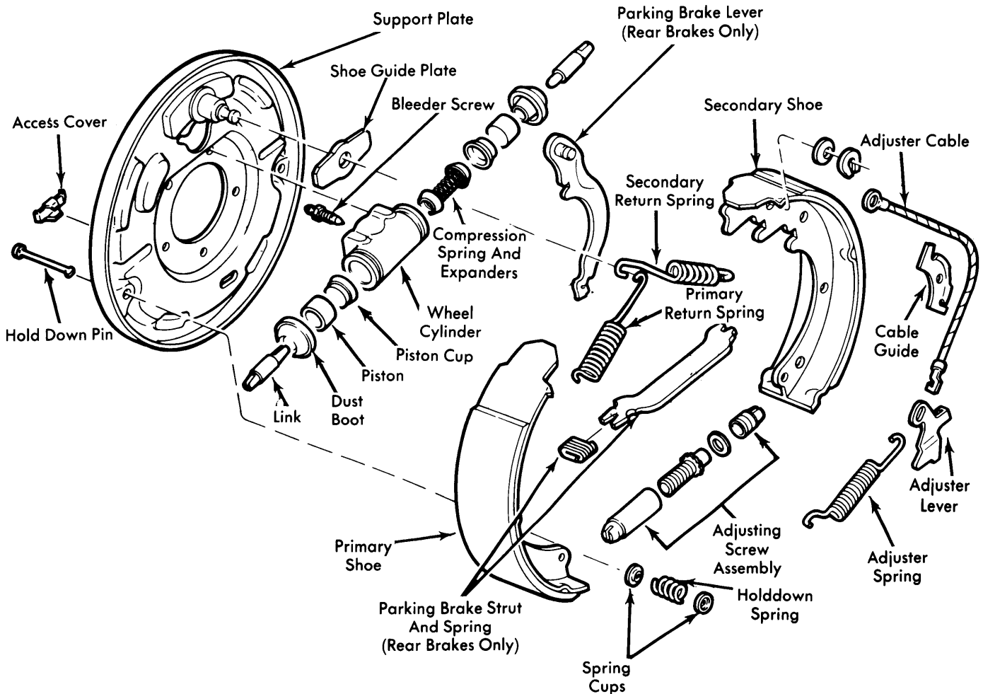
Fig. 1 Exploded View of Brake Assembly
