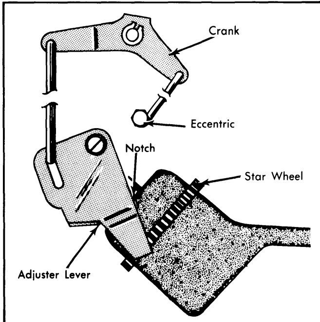
Fig. 2 Initial Adjustment to Manual Adjuster
