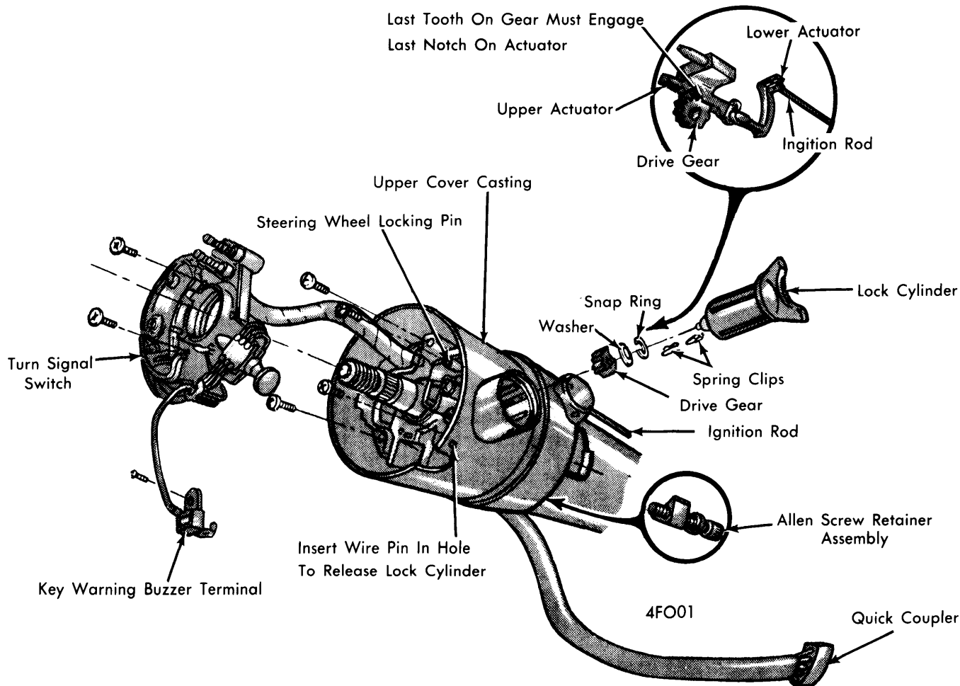
TILT COLUMN MECHANISM
