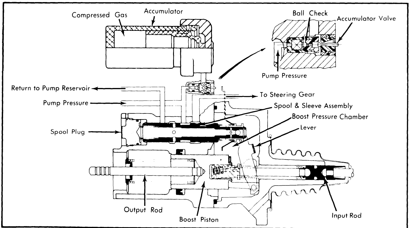
Fig. 5 Sectional View of Ford Motor Co. Hydro-Boost Hydraulic Circuits
