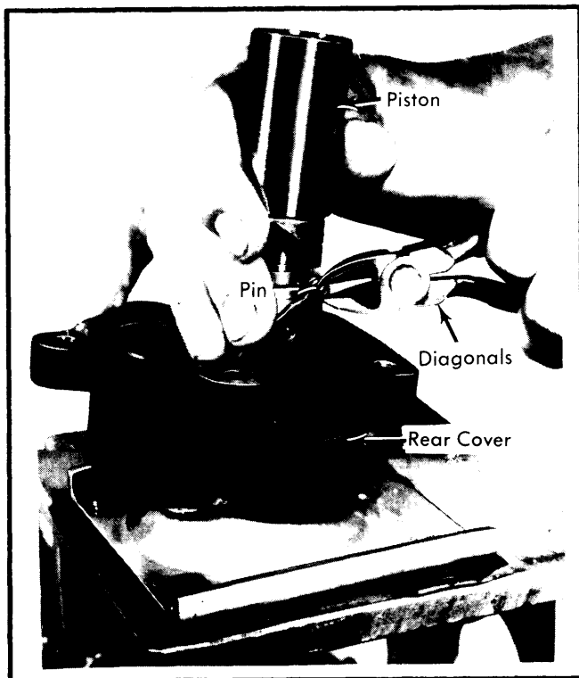
Fig. 9 Using Diagonal Cutters to Remove Booster Power Pin (Cadillac Shown)
