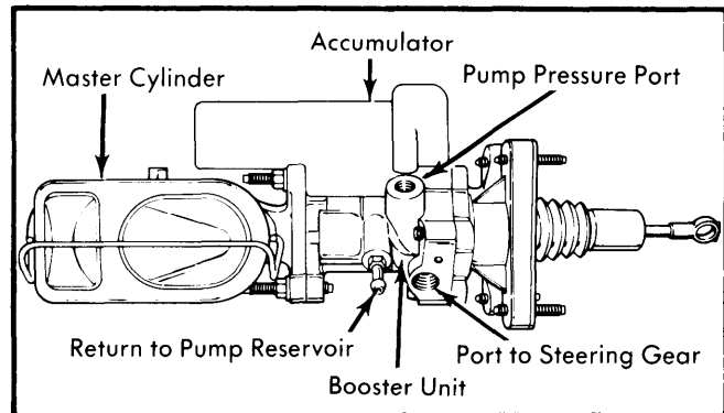
Fig. 2 Ford Motor Co. Hydro-Boost Power Brake Unit Used on Ford, Mercury, Lincoln, & Mark V
