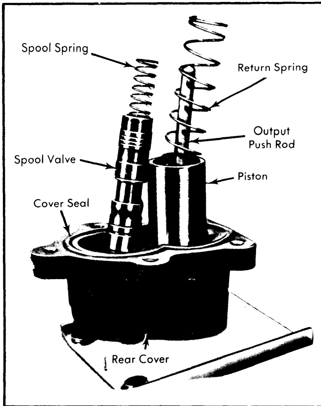
Fig. 8 Booster Rear Cover Assembly Showing Spool Valve & Power Piston (Cadillac Shown)
