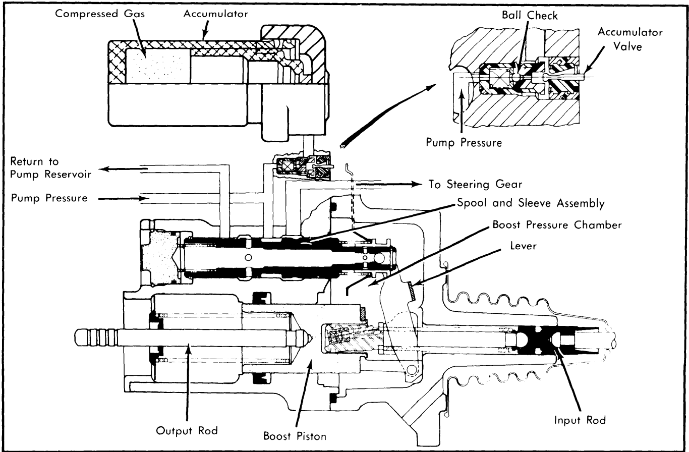
Fig. 4 Sectional View of Cadillac Hydro-Boost Hydraulic Circuits
