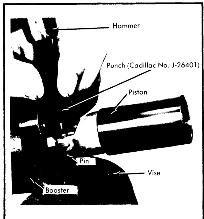
Fig. 10 Staking Booster Piston Pin (Cadillac Shown)
