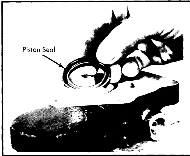
Fig. 11 Installing New Power Piston Seal into Rear Housing (Cadillac Shown)
