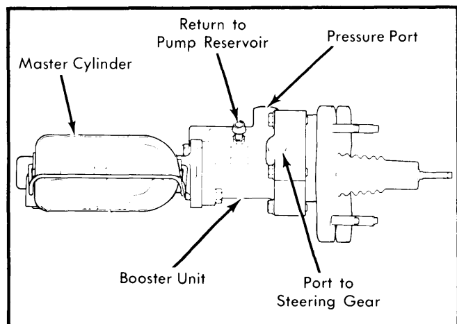
Fig. 3 Ford Motor Co. Hydro-Boost Power Brake Unit Used on Granada, Monarch, & Versailles
