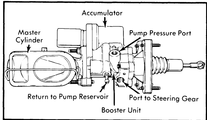
Fig. 1 Cadillac Hydro-Boost Power Brake Unit
