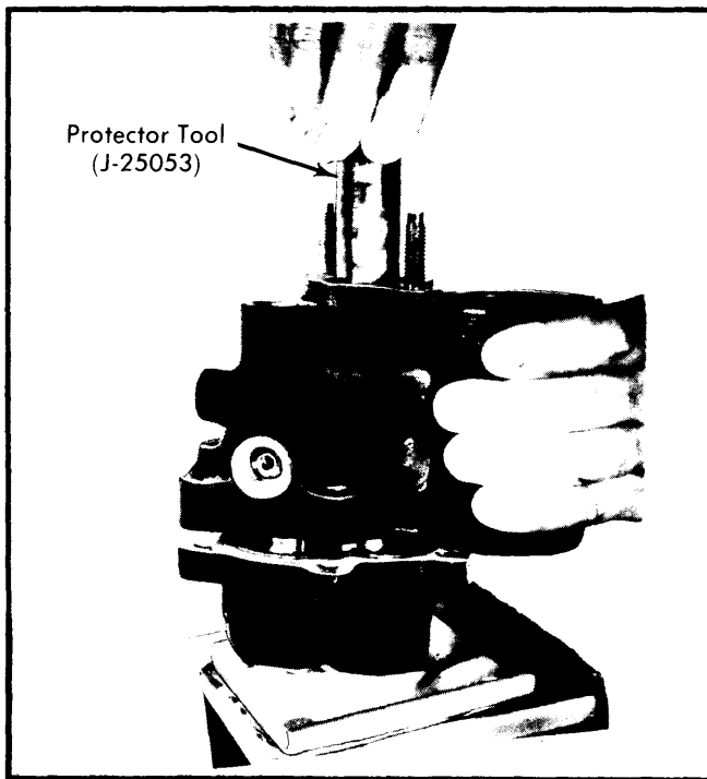
Fig. 12 Installing Seal Protector Tool Through Front Housing (Cadillac Shown)
