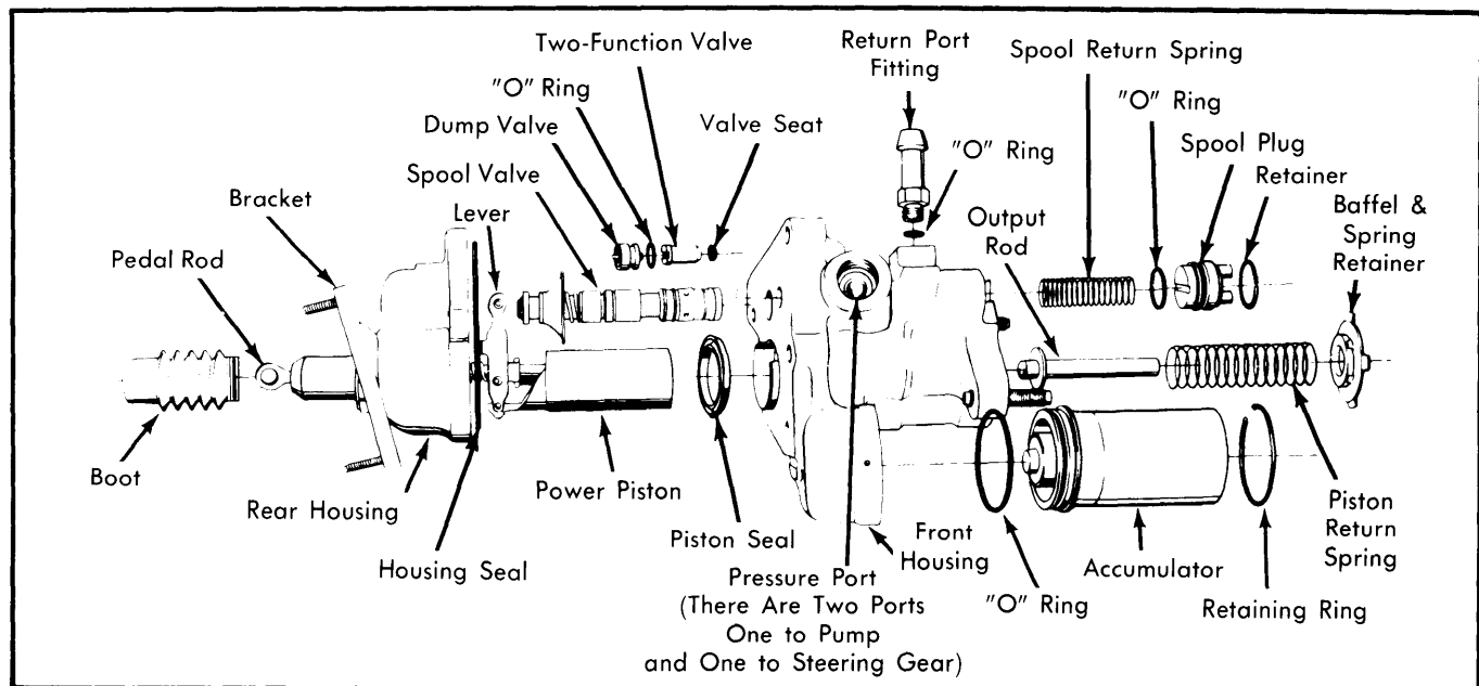
Fig. 6 Exploded View of Typical Hydro-Boost Power Brake System (Chevrolet Unit Shown)
