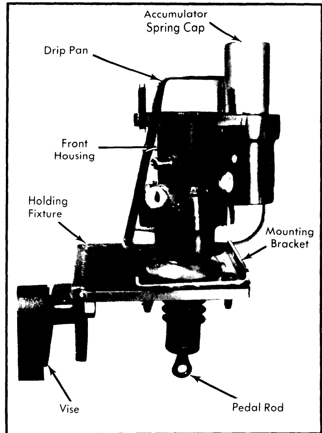
Fig. 7 Mounting Booster on Holding Fixture & Clamping Fixture in a Vise for Booster Disassembly (Cadillac Shown)
