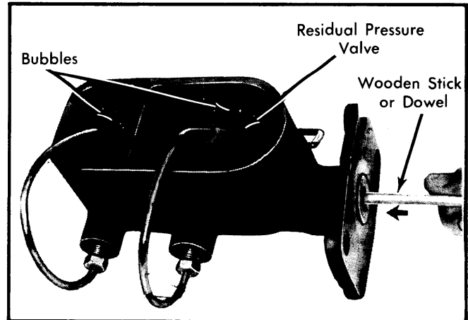
Fig. 1 Bleeding Master Cylinder With Bleeding Tubes Installed
