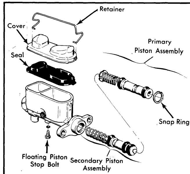
Fig. 3 Typical Bendix Master Cylinder (Ford Motor Co. Shown)
