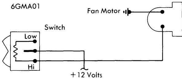
REAR WINDOW DEFOGGER WIRING DIAGRAM (RESISTOR-IN-SWITCH CIRCUIT - TYPICAL)
