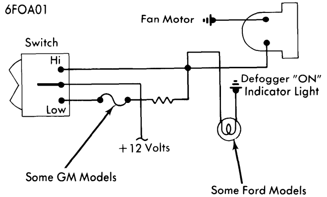
REAR WINDOW DEFOGGER WIRING DIAGRAM (RESISTOR-IN-LINE CIRCUIT - TYPICAL)
