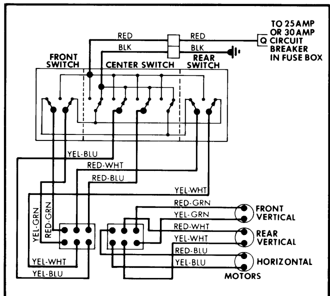
Fig. 2 Chrysler Power Seat Wiring Diagram
