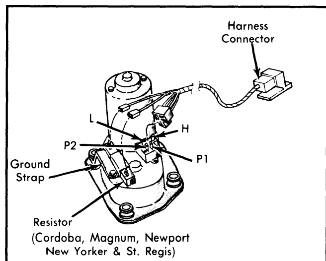
Fig. 1 Chrysler 2-Speed Motor Terminal Identification
