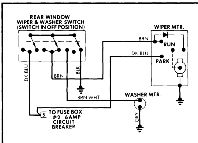
Fig. 6 Chrysler Tailgate Wiper System Wiring Diagram
