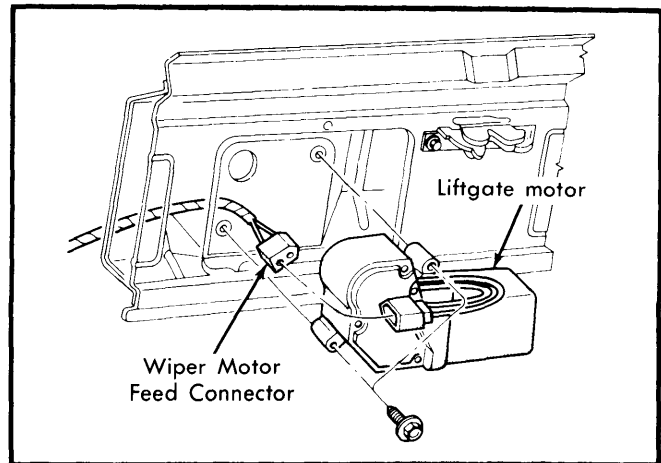
Fig. 7 View Showing Removal of Liftgate Motor
