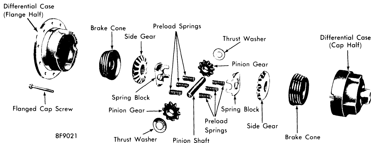
WARNER-MOTIVE DIFFERENTIAL ASSEMBLY (TYPICAL)
