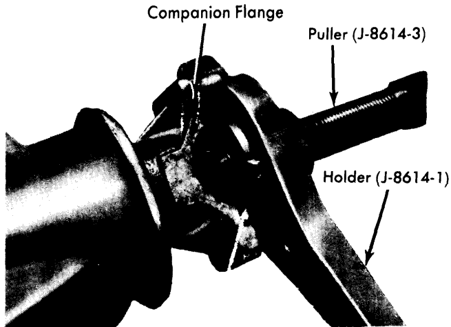
Fig. 2 Typical Removal of Companion Flange
