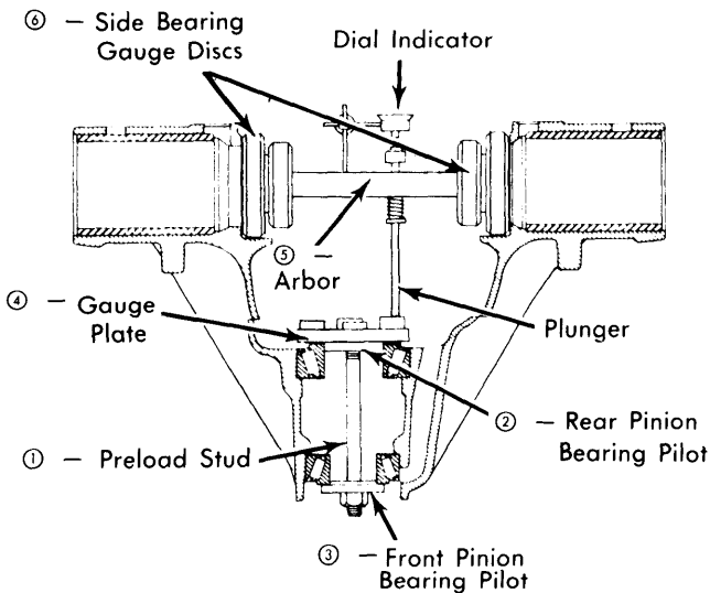
Fig. 6 Special Tool Assembly (Typical)
