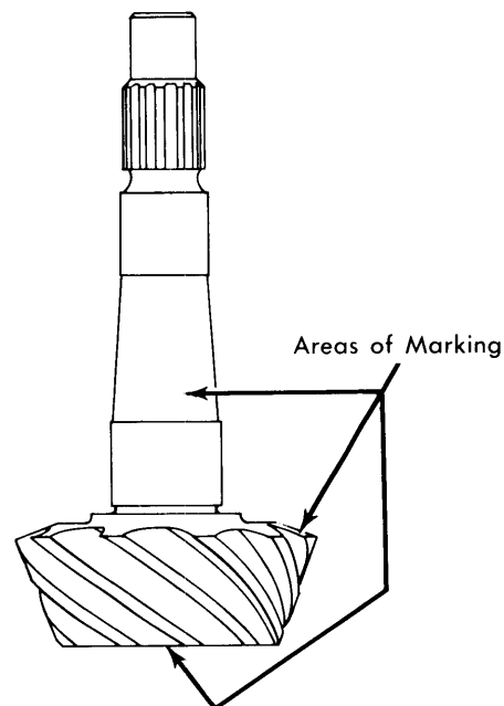
Fig. 5 Pinion Marking Locations
