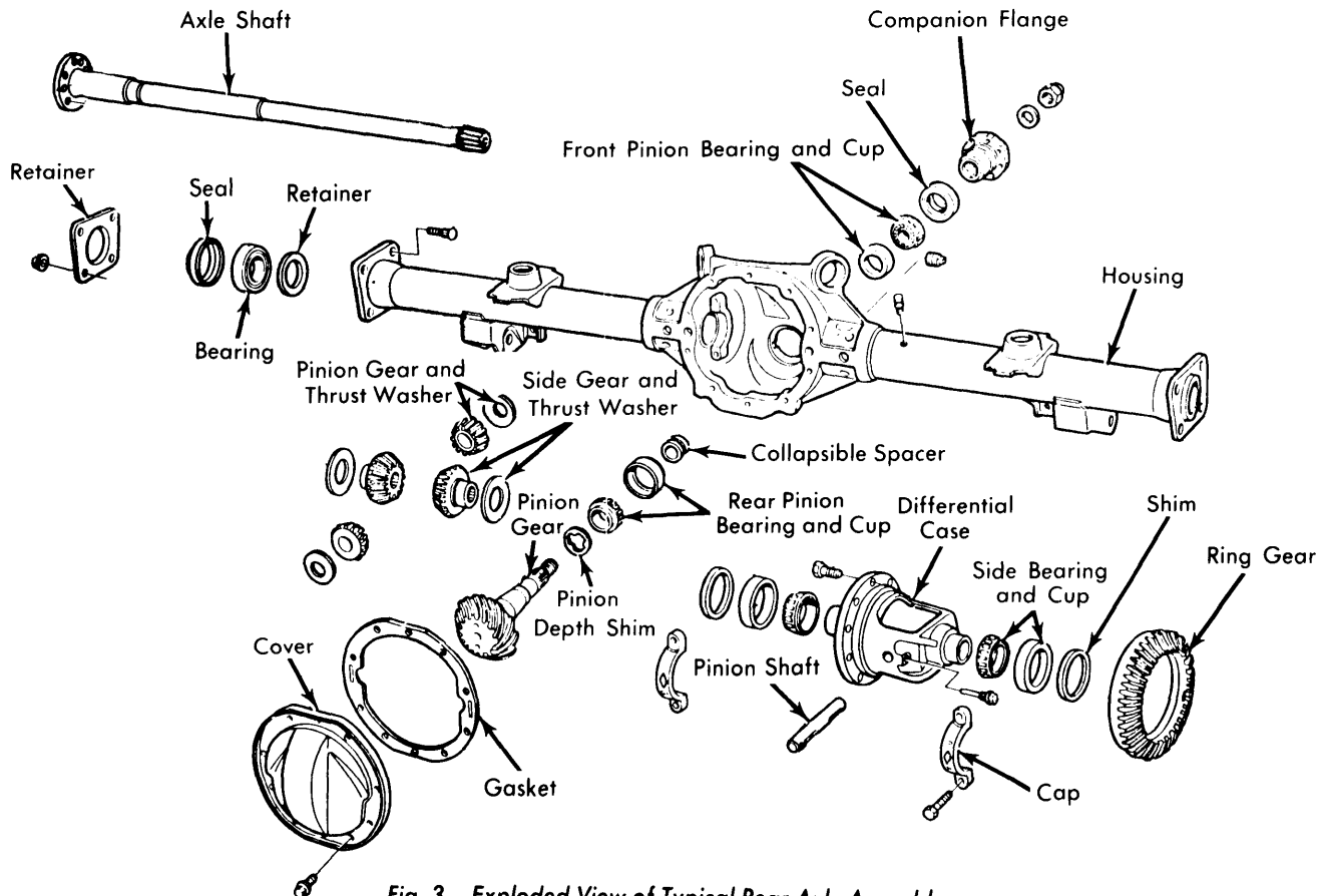
Fig. 3 Exploded View of Typical Rear Axle Assembly
