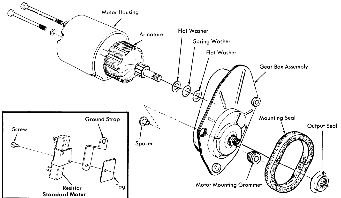
Fig. 3 Exploded View 2-Speed Wiper Motor
