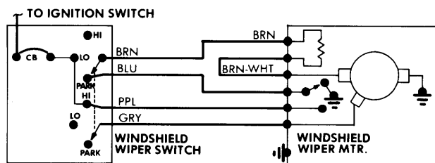
Fig. 2 Chrysler 2-Speed Wiper Wiring Diagram
