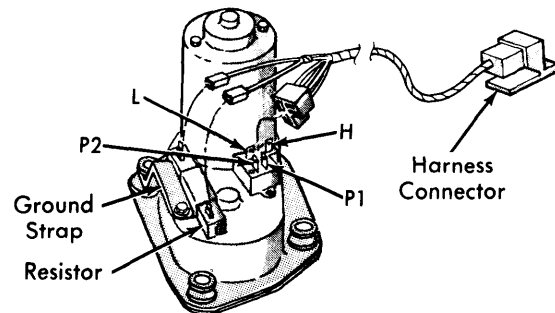
Fig. 1 2-Speed Wiper Motor Terminal Identification
