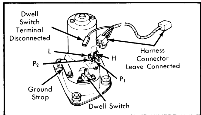
Fig. 1 Two Speed Intermittent Wiper Motor Terminal Identification (Standard Terminal Similar)
