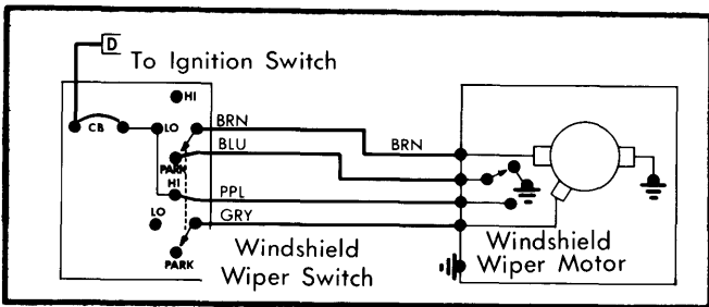
Fig. 2 Chrysler 2-Speed Wiper Wiring Diagram
