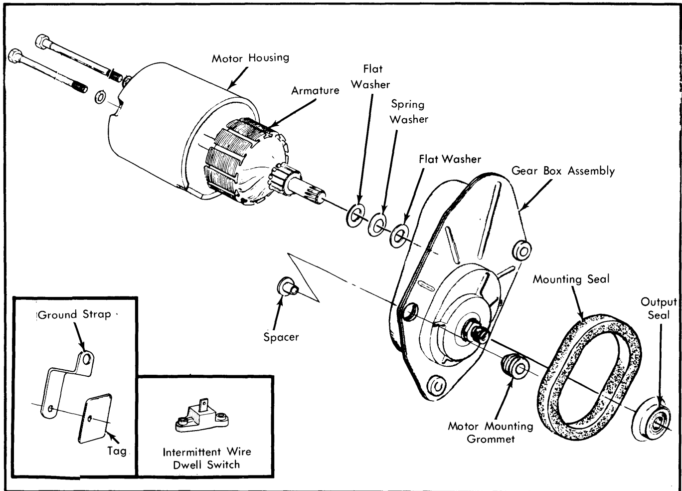
Fig. 4 Wiper Motor Exploded View
