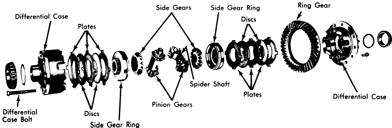
Fig. 1 Exploded View of Dana/Spicer Power-Lok Differential Assembly
