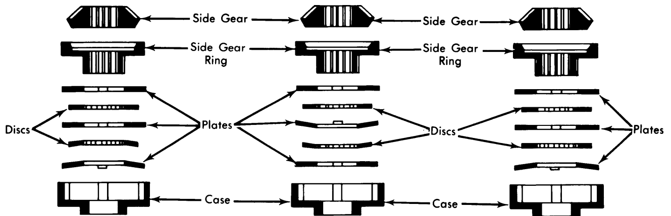
Fig. 2 Three Views Showing Typical Clutch Pack Arrangements (Not All Combinations are Shown)
