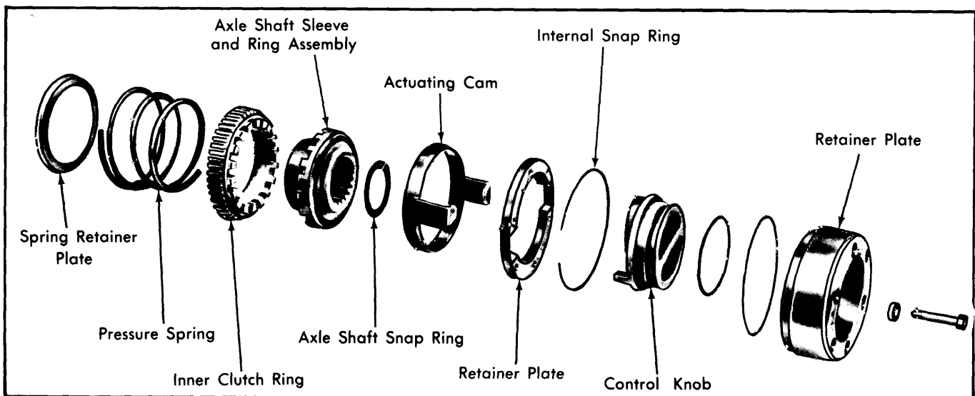
Fig. 2 Exploded View of Dana/Spicer 6 Bolt Locking Hub
