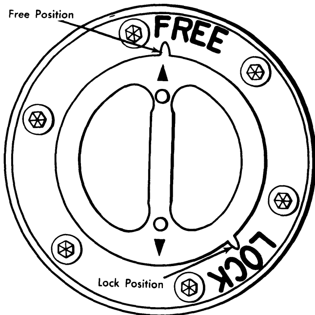
Fig. 1 Front View of Dana/Spicer Locking Hub
