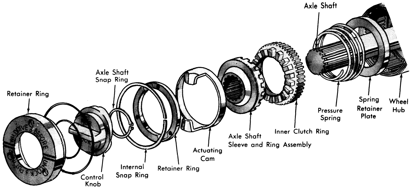
Fig. 3 Exploded View of Dana/Spicer 3 Bolt Locking Hub
