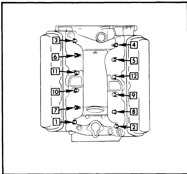
Fig. 1 Intake Manifold Tightening Sequence
