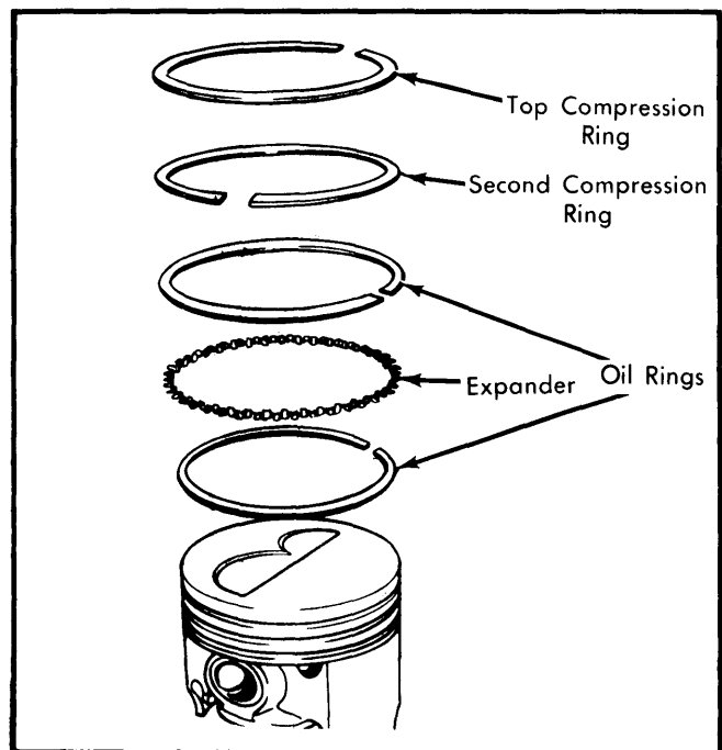
Fig. 7 Piston Rings
