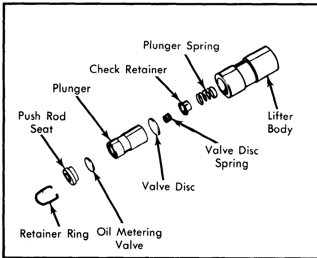
Fig. 6 Valve Lifter
