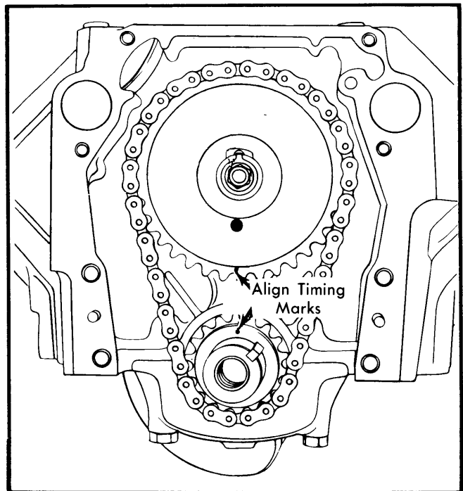
Fig. 11 Aligning Timing Marks
