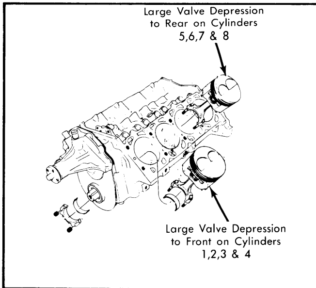
Fig. 8 Piston Location
