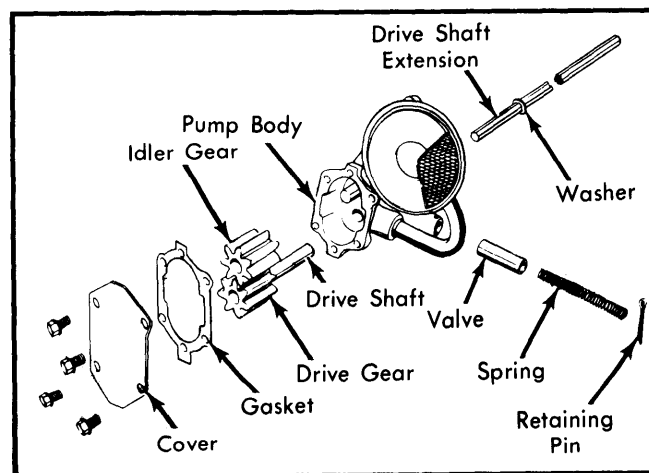
Fig. 13 Oil Pump
